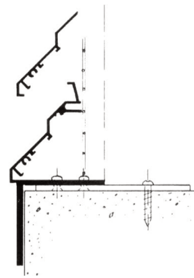
Type CEL50/75/100 Surface Frame with Strap-type Fixing
