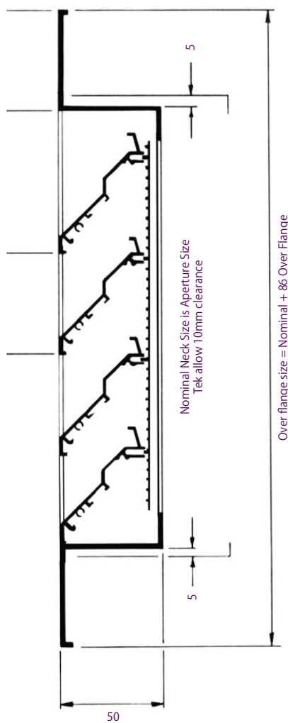
Type CEL50/75/100 Surface Frame Typical Installation
