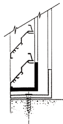
Type LD50/75/100 Recess Frame
