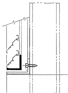
Type LD50/75/100 Recess Frame
