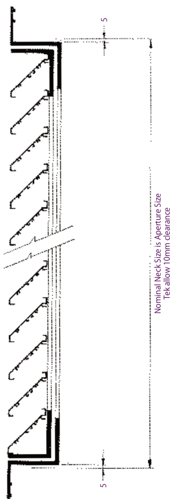
Type LD50/75/100 Typical Installation
